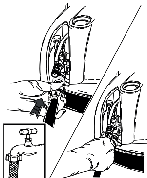
Raccordement hydraulique.
